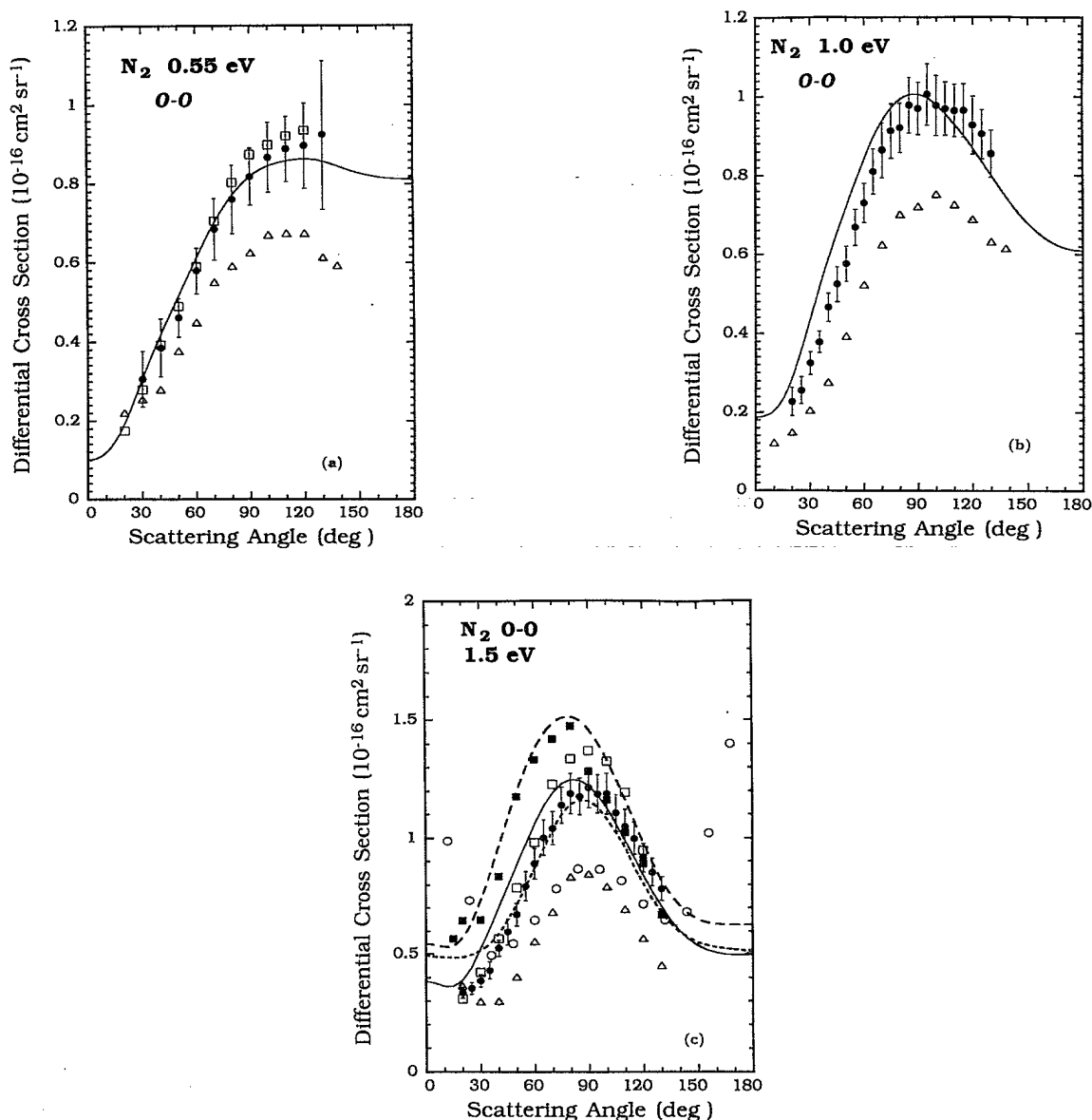
FIG. 7. Absolute elastic differential cross sections at energies of (a) 0.55 eV, (b) 1.0 eV, and (c) 1.5 eV. In addition to the present experimental (solid circles) and theoretical (solid lines) results, we show the data of Sohn et al. [54] (open triangles) and in (a) and (c) of Shi, Stephen, and Burrow [58] (open squares). Also shown in (c) are measured DCSs of Shyn and Carignan [45] (open circles) and the hybrid-theory results of Chandra and Temkin [34] (long-dashed line) and Schwinger multichannel DCSs of Huo et al. [30] (short-dashed line).
