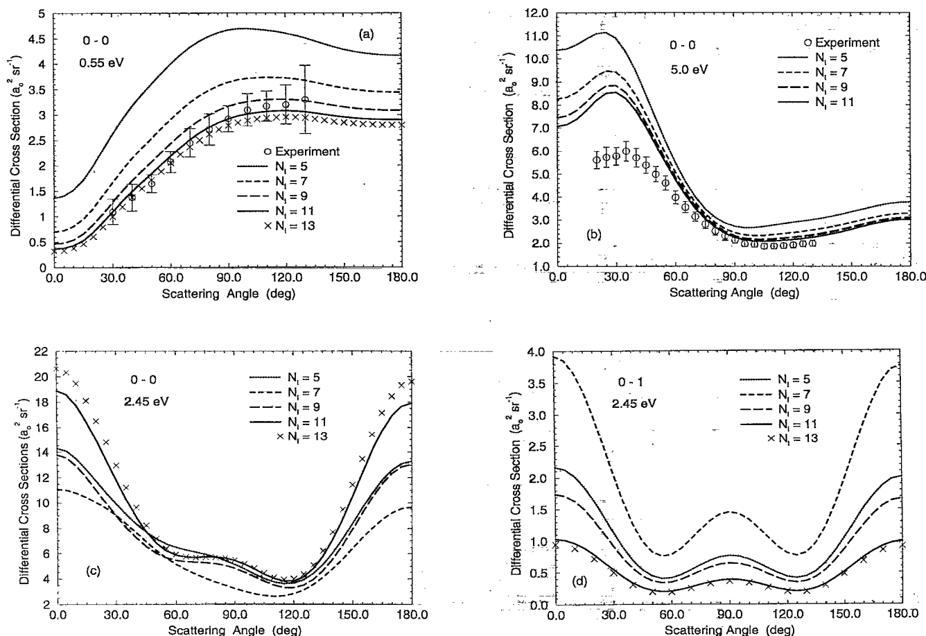
FIG. 2. Convergence in the number of partial waves N_l in the near-target region of the elastic e\text{-N}_2 DCS at (a) 0.55 eV, (b) 5.0 eV, and (c) 2.45 eV and of (d) the 0 \rightarrow 1 DCS at 2.45 eV. These results are converged in vibrational states in Eq. (8) and in asymptotic partial waves and symmetries in the Legendre coefficients of the DCS, Eq. (3). The experimental data (open circles) in (a) and (b) are from the present crossed-beam measurements.
