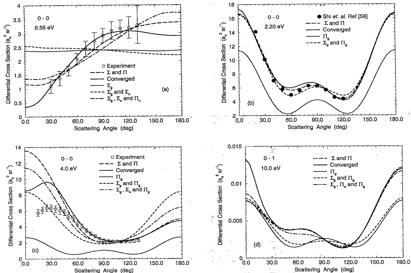
FIG. 3. Convergence in the number of electron-molecule symmetry classes included in the Legendre coefficients of the DCS for the elastic e\text{-N}_2 DCSs at (a) 0.55 eV, (b) 2.2 eV, and (c) 4.0 eV and of (d) the 0\rightarrow 1 DCSs at 10.00 eV. These results are converged in vibrational states and partial waves in the near-target region [see Eq. (8)]. The results designated “converged” (solid line) contain contributions from the first 16 symmetry classes. The experimental data (open circles) are from the present crossed-beam measurements.
