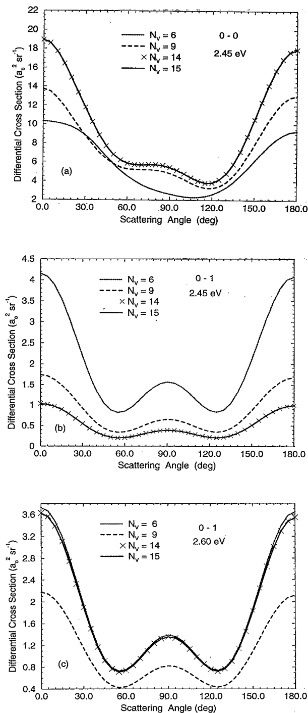
FIG. 1. Convergence in the number of vibrational states N_v of (a) the elastic e\text{-N}_2 DCS at 2.45 eV and the inelastic DCS at (b) 2.45 eV and (c) 2.60 eV. These results are converged in partial waves in the near-target region [see Eq. (8)] and in asymptotic partial waves and symmetries in the Legendre coefficients (3) of the DCS.
