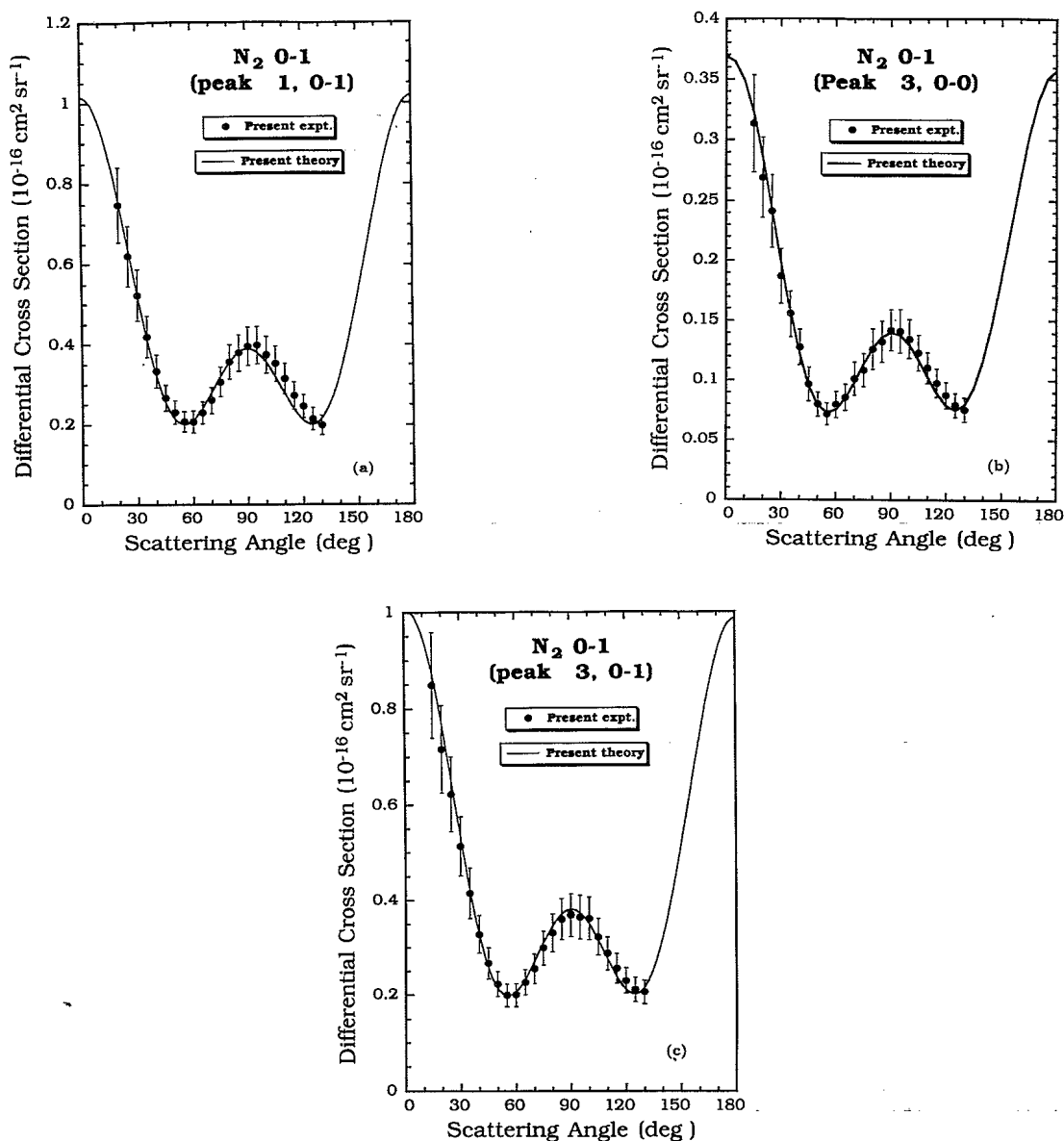
FIG. 5. Absolute DCS for vibrational excitation of N_2 at the position of (a) the first resonance peak in the 0 \rightarrow 1 channel, (b) the third resonance peak in the 0 \rightarrow 0 channel, and (c) the third resonance peak in the 0 \rightarrow 1 channel, all determined at 60^\circ : theoretical DCSs (solid line), measured DCSs (closed circles).
