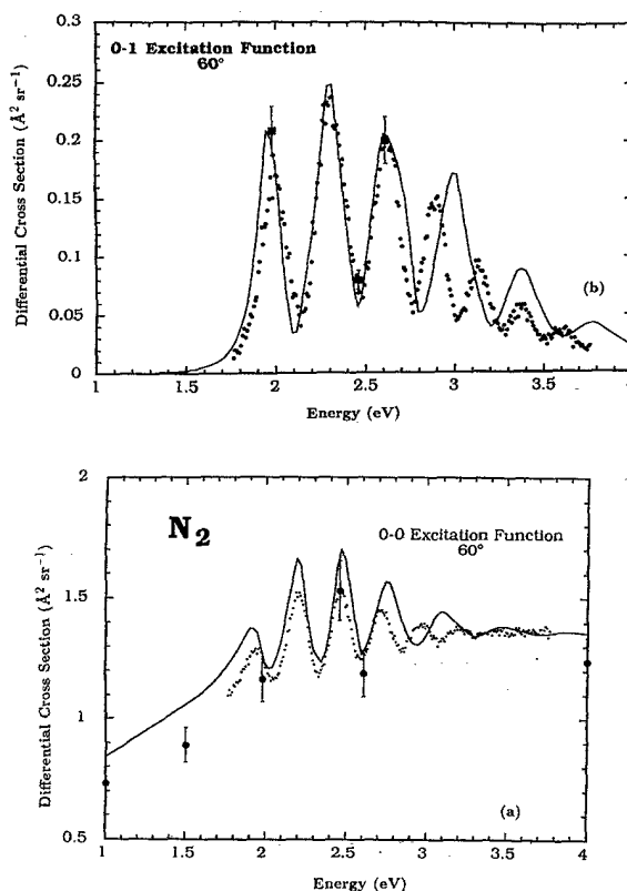
FIG. 4. Energy dependence of the (a) elastic and (b) inelastic ( 0 \rightarrow 1 ) DCSs from theoretical (solid line) calculations compared to measured excitation functions (dots) and DCS data (solid circles).
